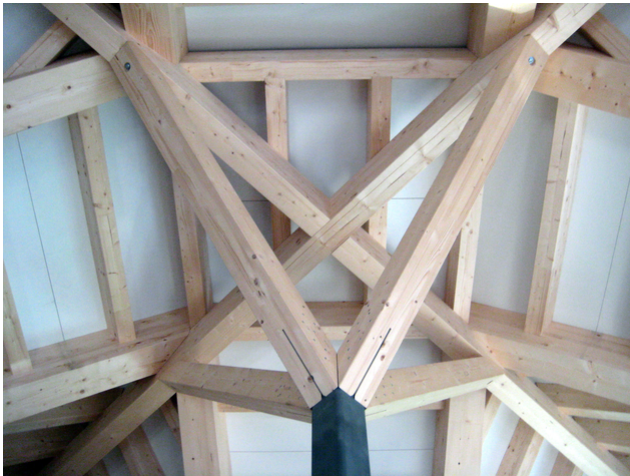
Roof construction 2
