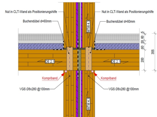
Detail Innen
