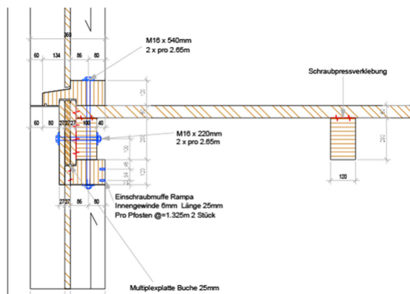
Connection detail: outer wall-floor slab
